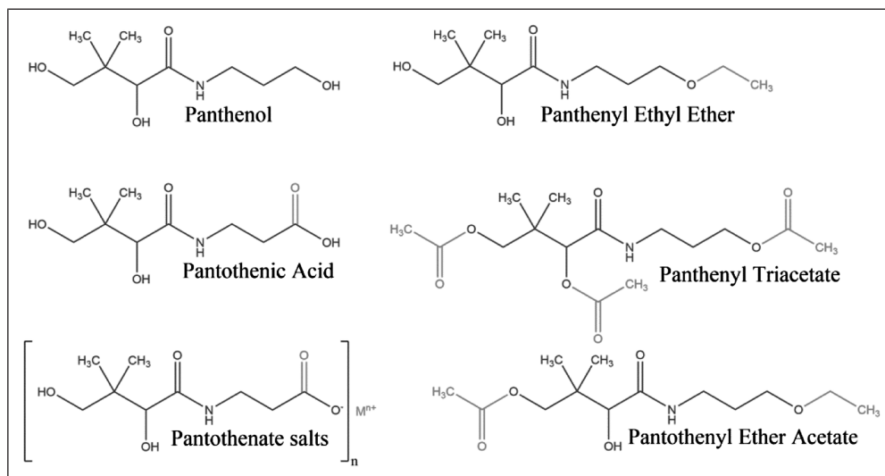
Figure 1. Panthenol, pantothenic acid, and derivatives.
